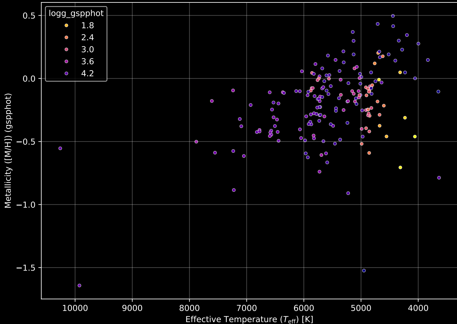
APOGEE DR17 Field: [053+32_MGA] Stellar Population Parameters (n= 181)
