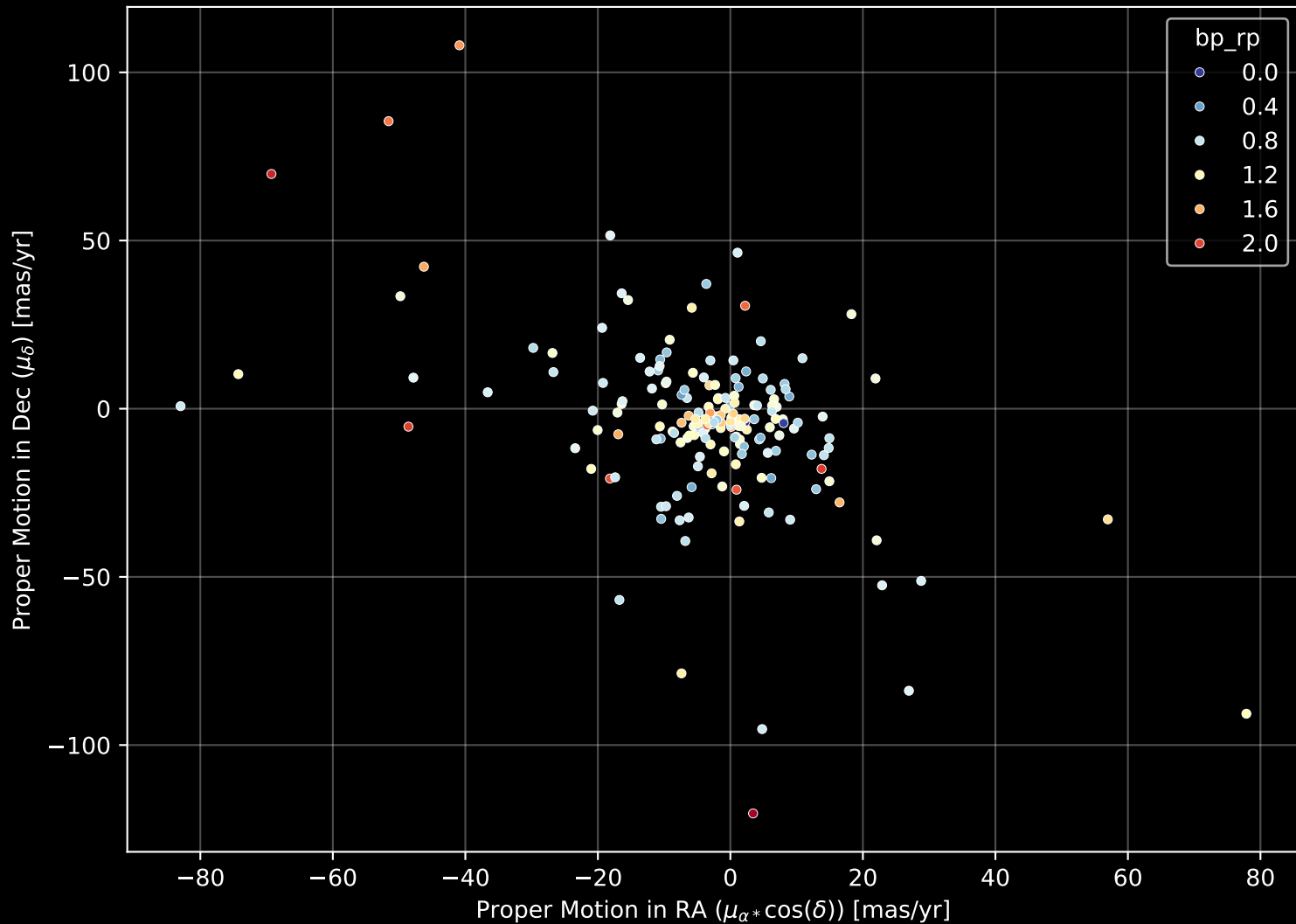
APOGEE DR17 Field: [053+32_MGA] Proper Motion Diagram (n= 181)
