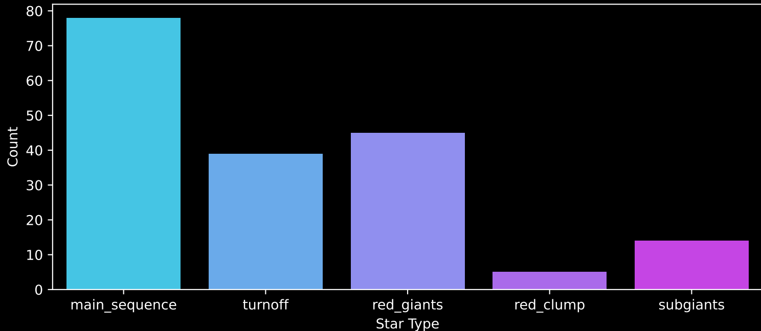
APOGEE DR17 Field: [053+32_MGA] Count plot of Star Type
