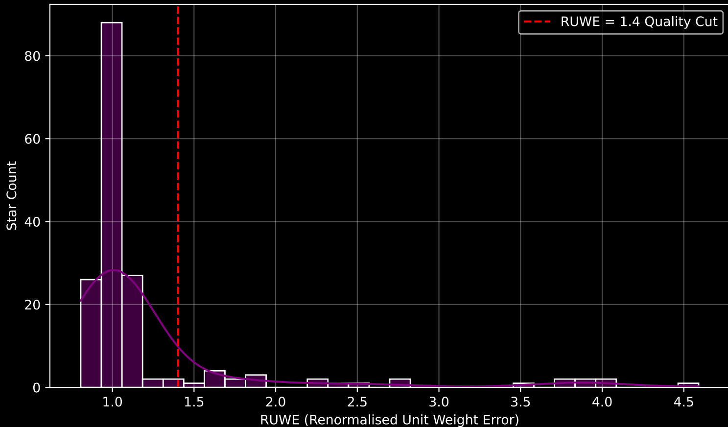
GAPOGEE DR17 Field [053+32_MGA] RUWE Distribution (n= 169)
