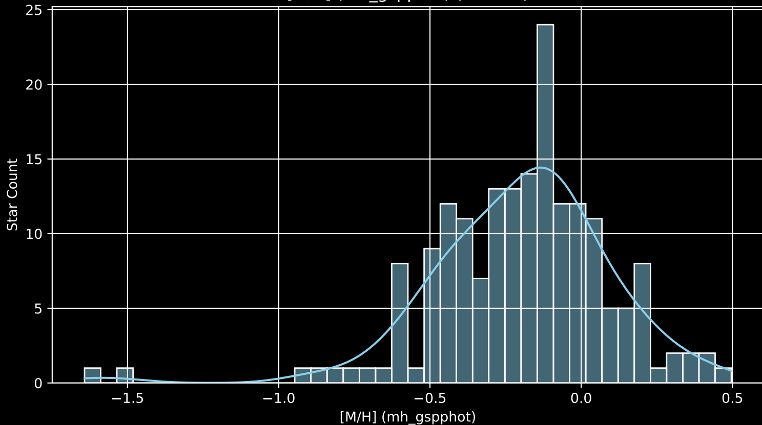
APOGEE DR17 Field: [053+32_MGA [M/H] (mh_gspphot) (n= 181)
