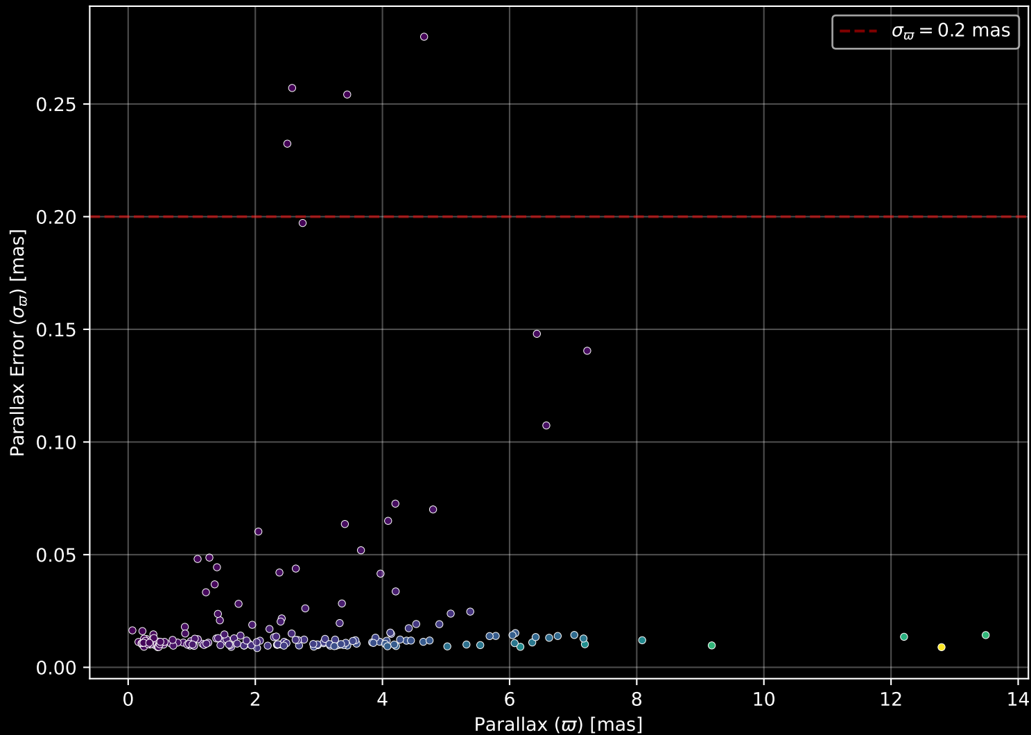
APOGEE DR17 Field: [053+32_MGA] Parallax Quality (n= 181)
